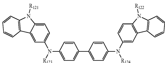
Formula 301
