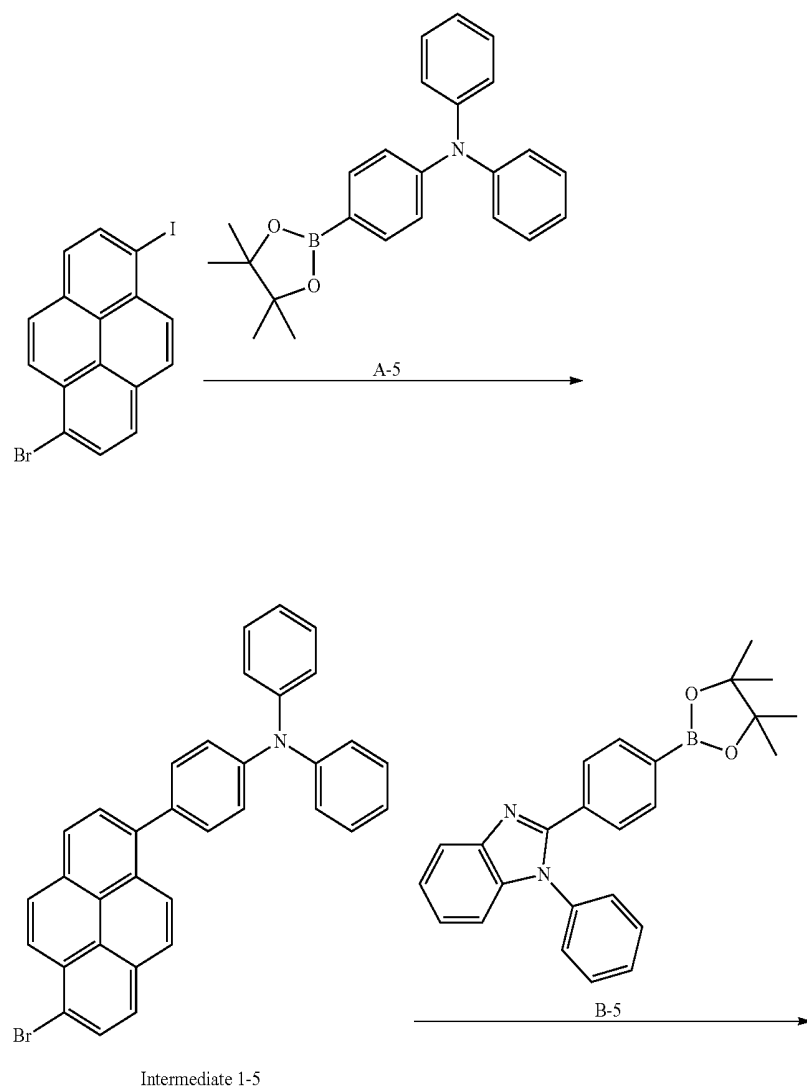
Reaction Scheme 1
