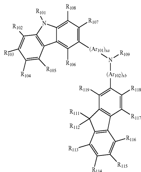
Formula 300
