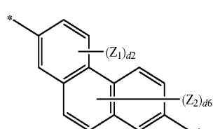
Formula 2-26
